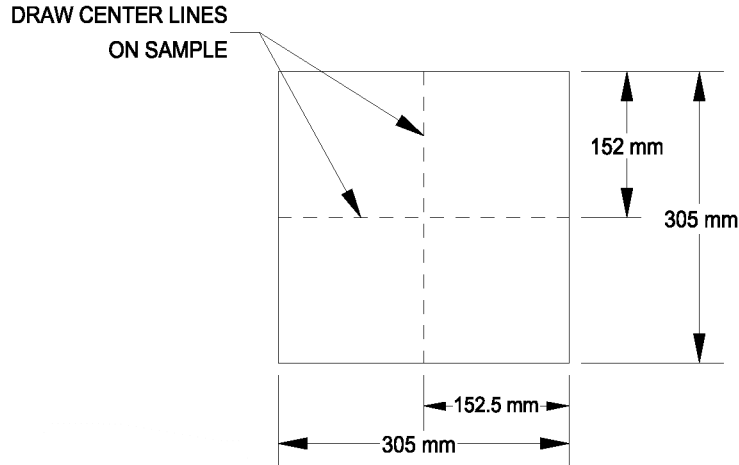
Figure 5: Sample Marking
